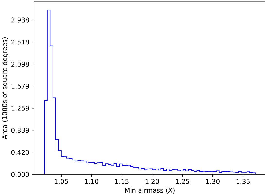
too_ignore_5_4v3.4_10yrs WFD y band: Min airmass
