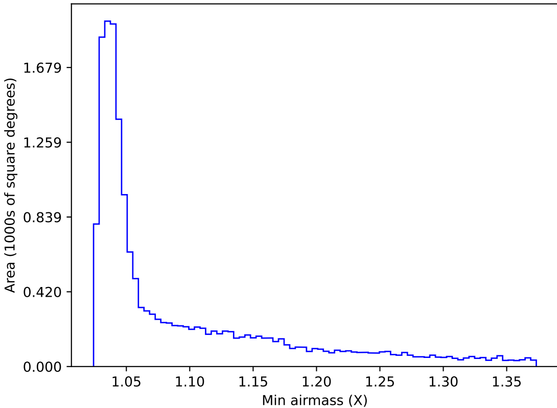
too_ignore_5_4v3.4_10yrs WFD u band: Min airmass
