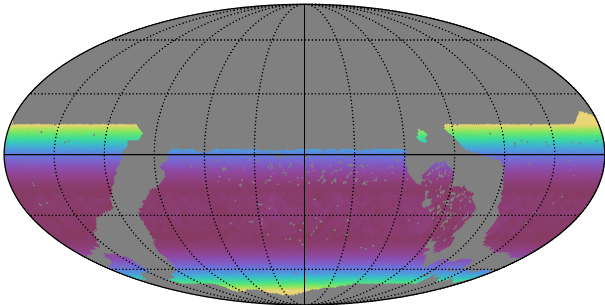
too_ignore_5_4v3.4_10yrs WFD r band: Min airmass
