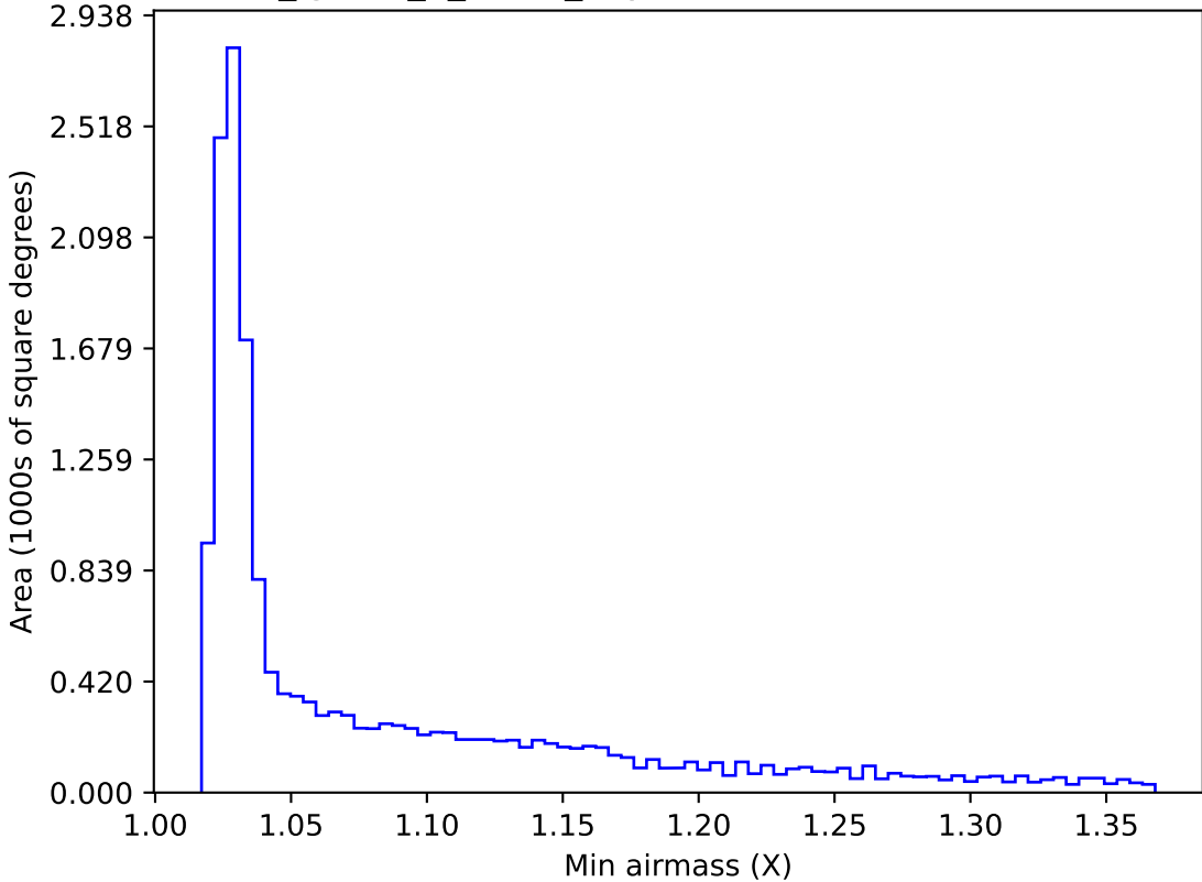
too_ignore_5_4v3.4_10yrs WFD r band: Min airmass
