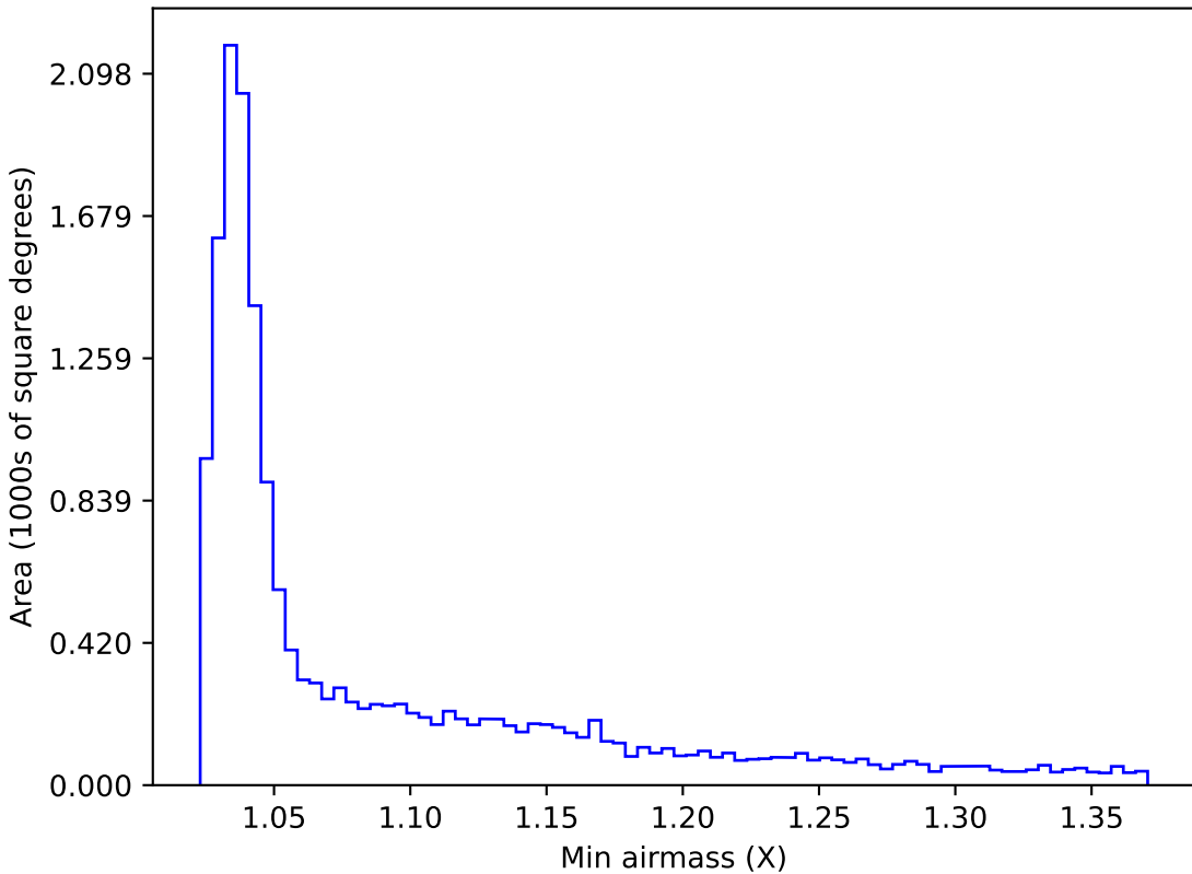
too_ignore_5_4v3.4_10yrs WFD g band: Min airmass
