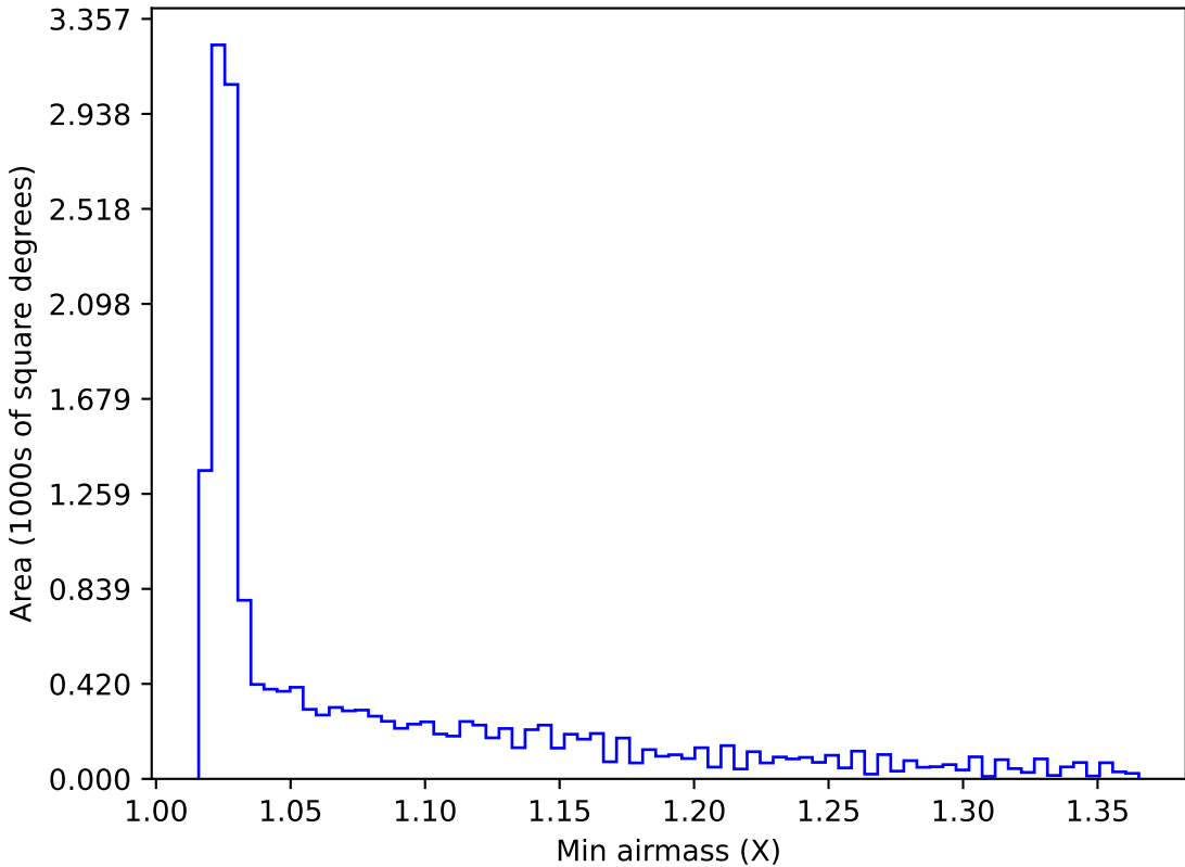
too_ignore_5_4v3.4_10yrs WFD all bands: Min airmass
