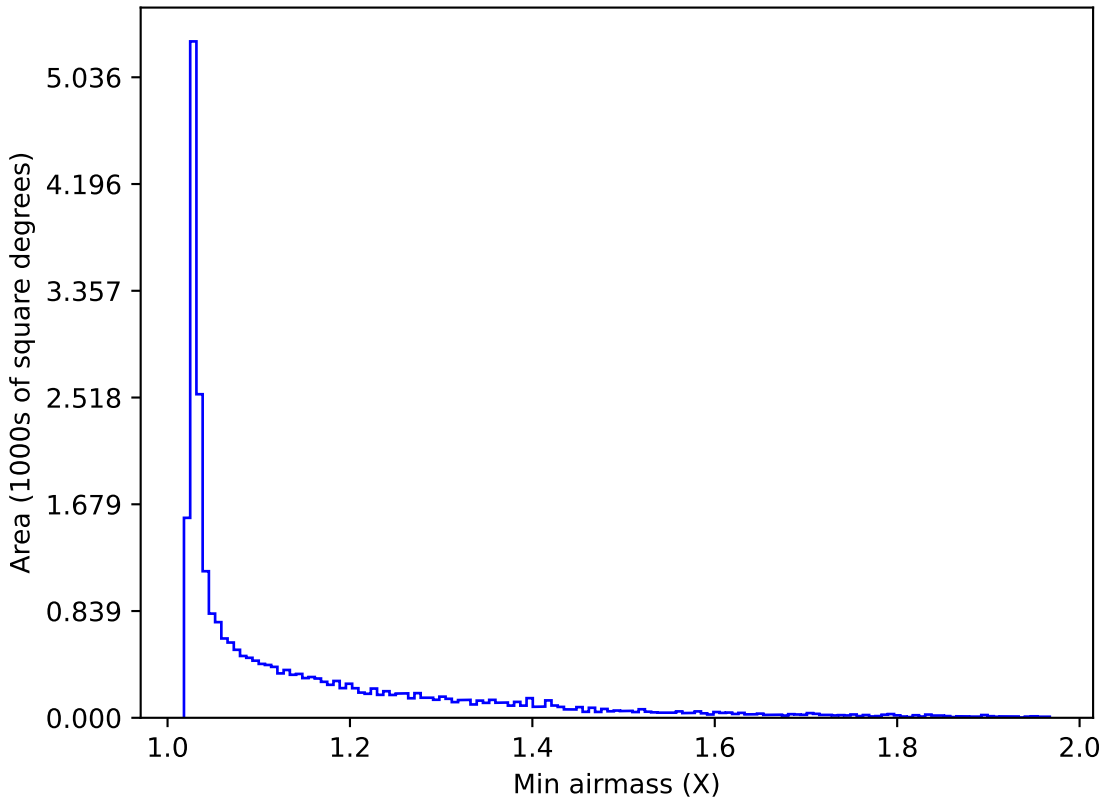
too_ignore_5_4v3.4_10yrs All sky z band: Min airmass
