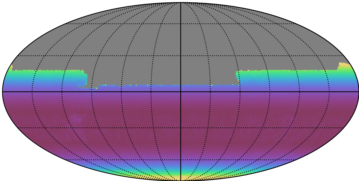
too_ignore_5_4v3.4_10yrs All sky y band: Min airmass
