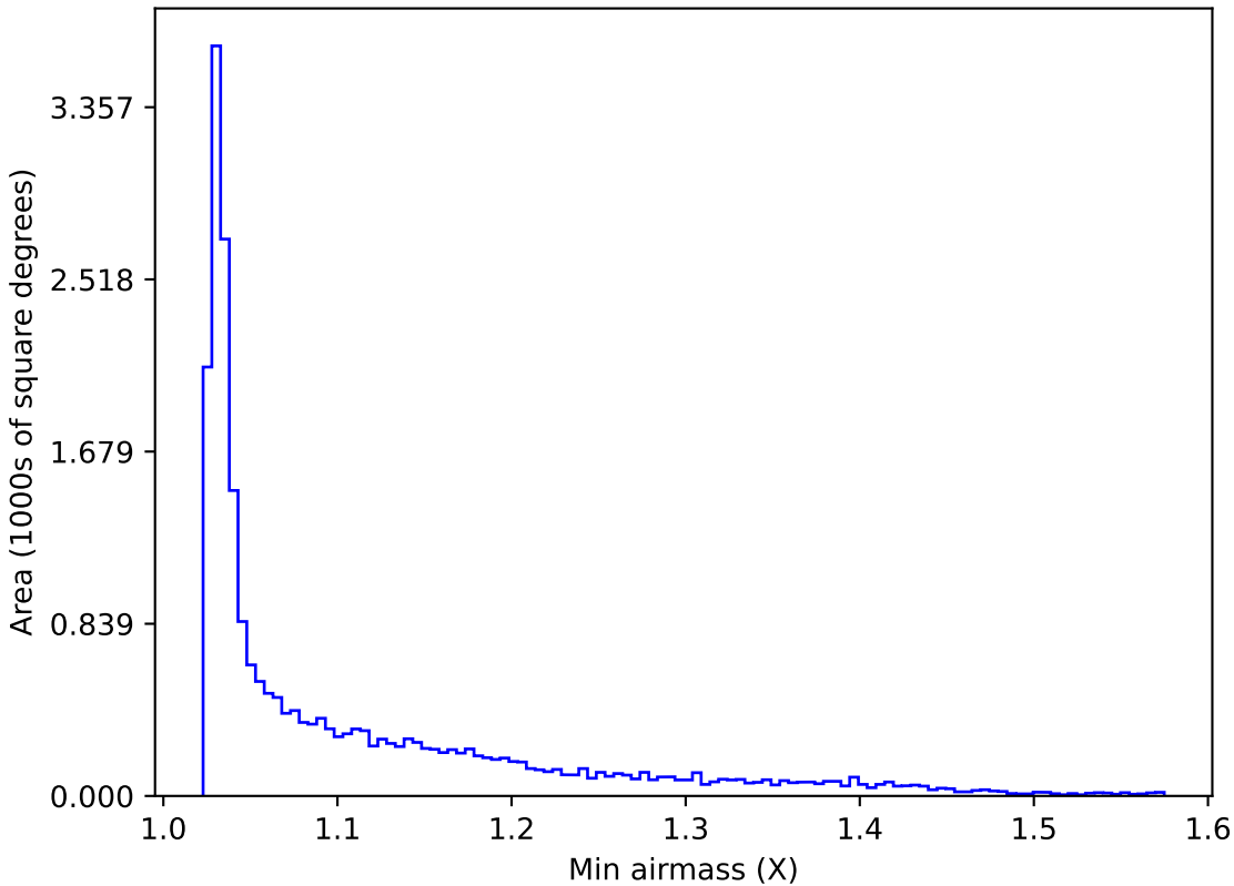
too_ignore_5_4v3.4_10yrs All sky y band: Min airmass
