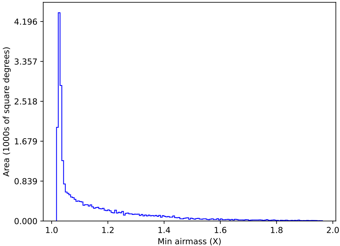
too_ignore_5_4v3.4_10yrs All sky r band: Min airmass
