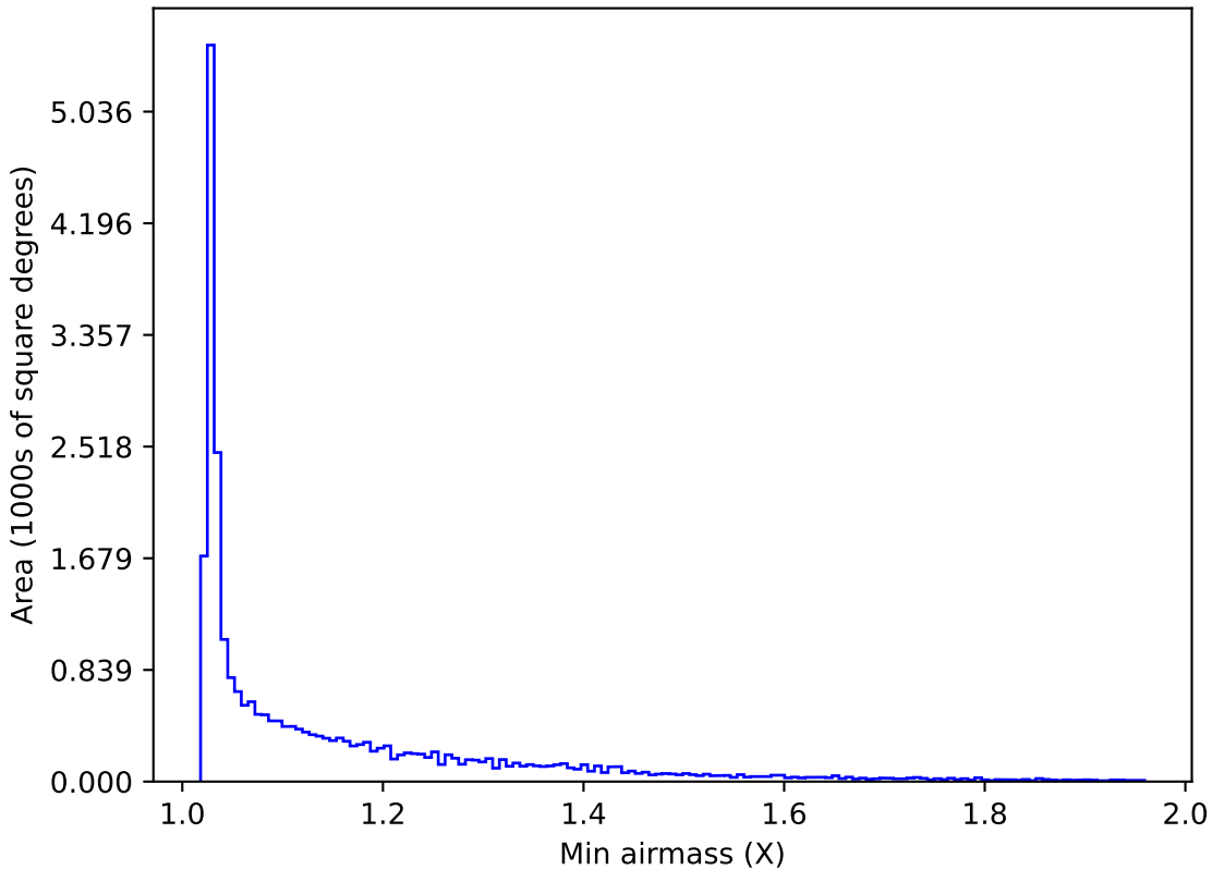
too_ignore_5_4v3.4_10yrs All sky i band: Min airmass
