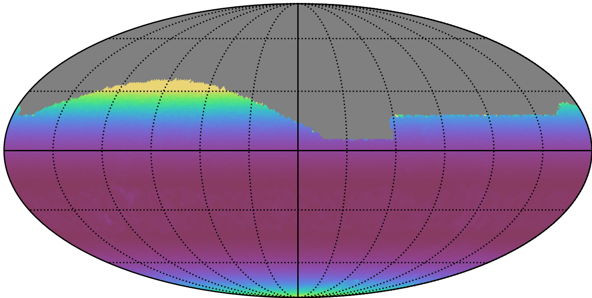
too_ignore_5_4v3.4_10yrs All sky g band: Min airmass
