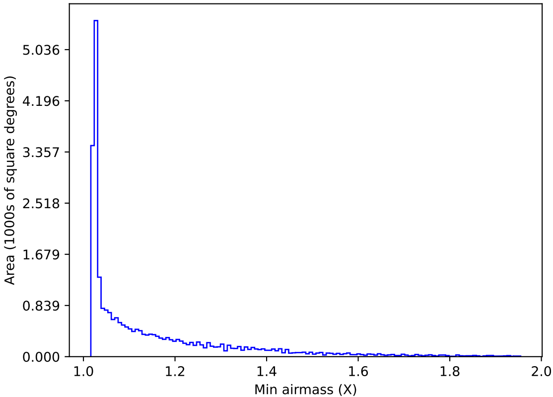
too_ignore_5_4v3.4_10yrs All sky all bands: Min airmass
