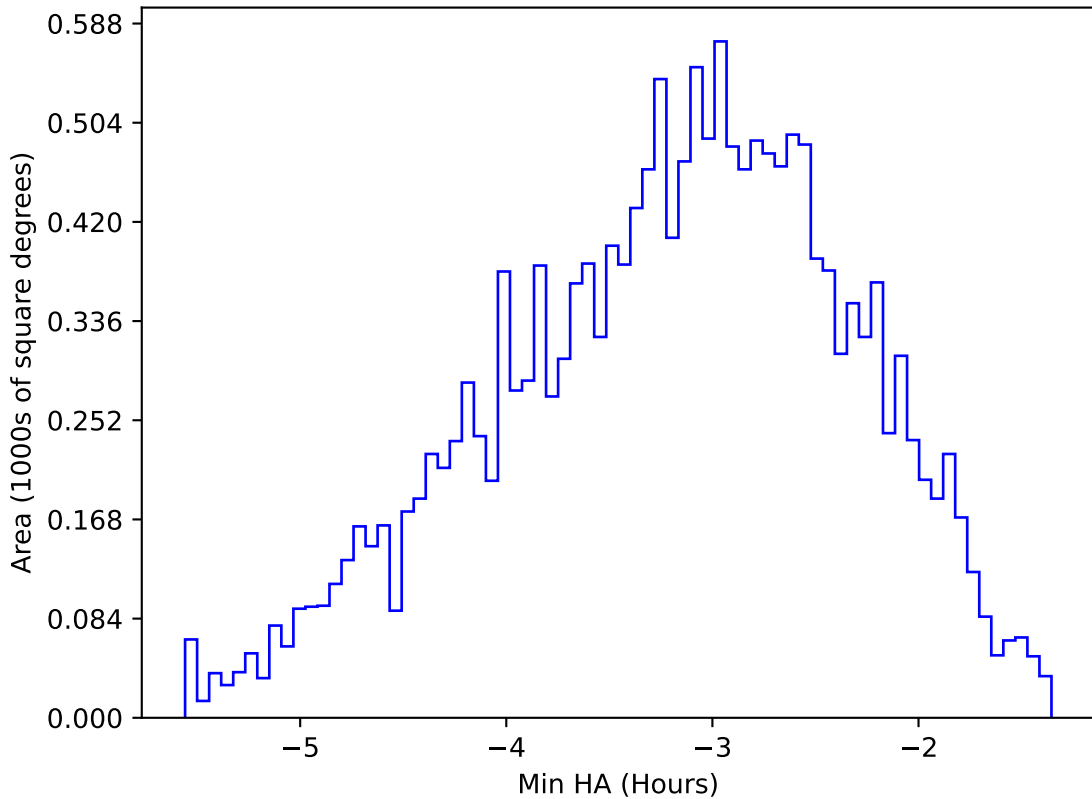
too_ignore_5_4v3.4_10yrs WFD u band: Min HA
