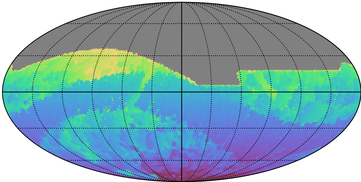
too_ignore_5_4v3.4_10yrs All sky r band: Min HA
