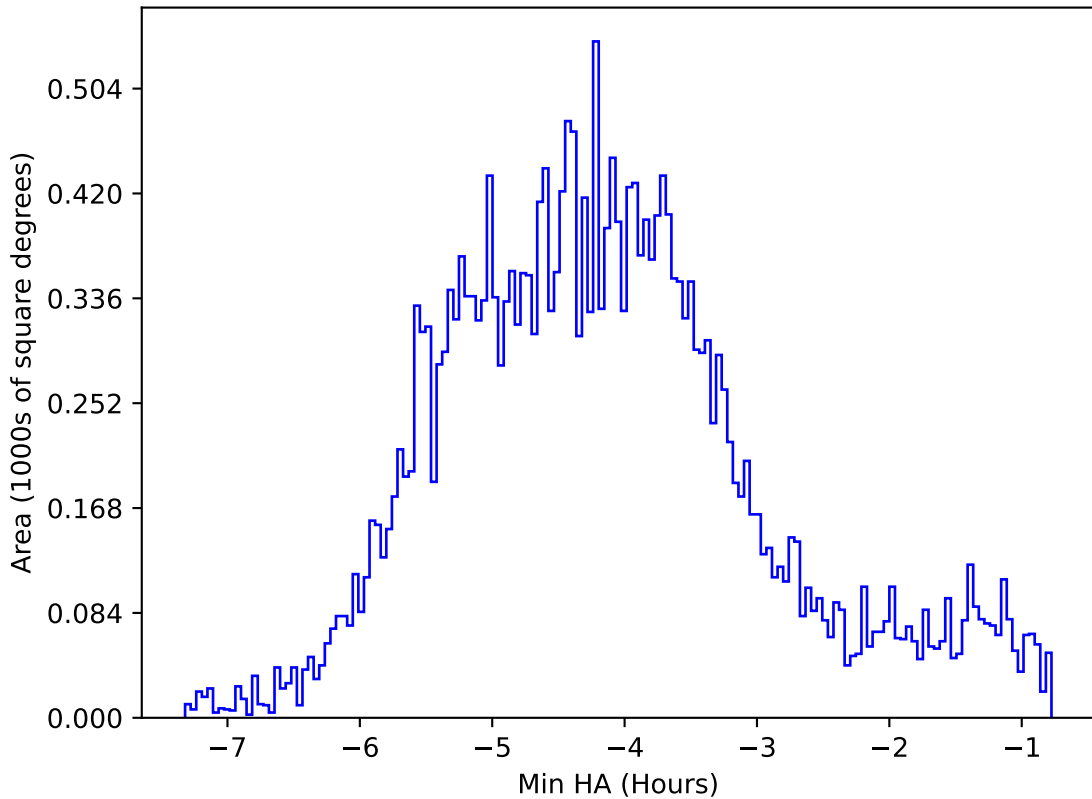
too_ignore_5_4v3.4_10yrs All sky r band: Min HA
