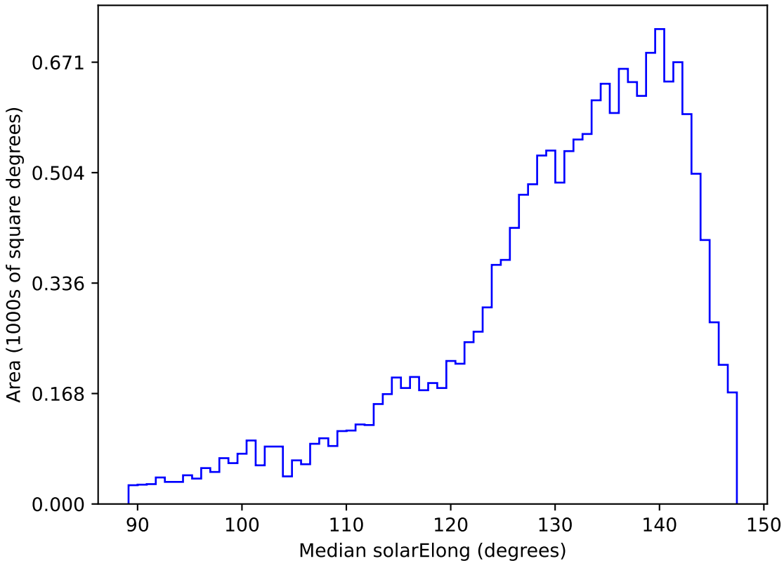
too_ignore_5_4v3.4_10yrs WFD y band: Median solarElong
