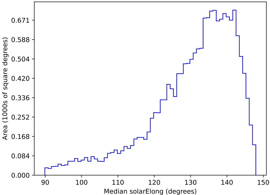
too_ignore_5_4v3.4_10yrs WFD r band: Median solarElong
