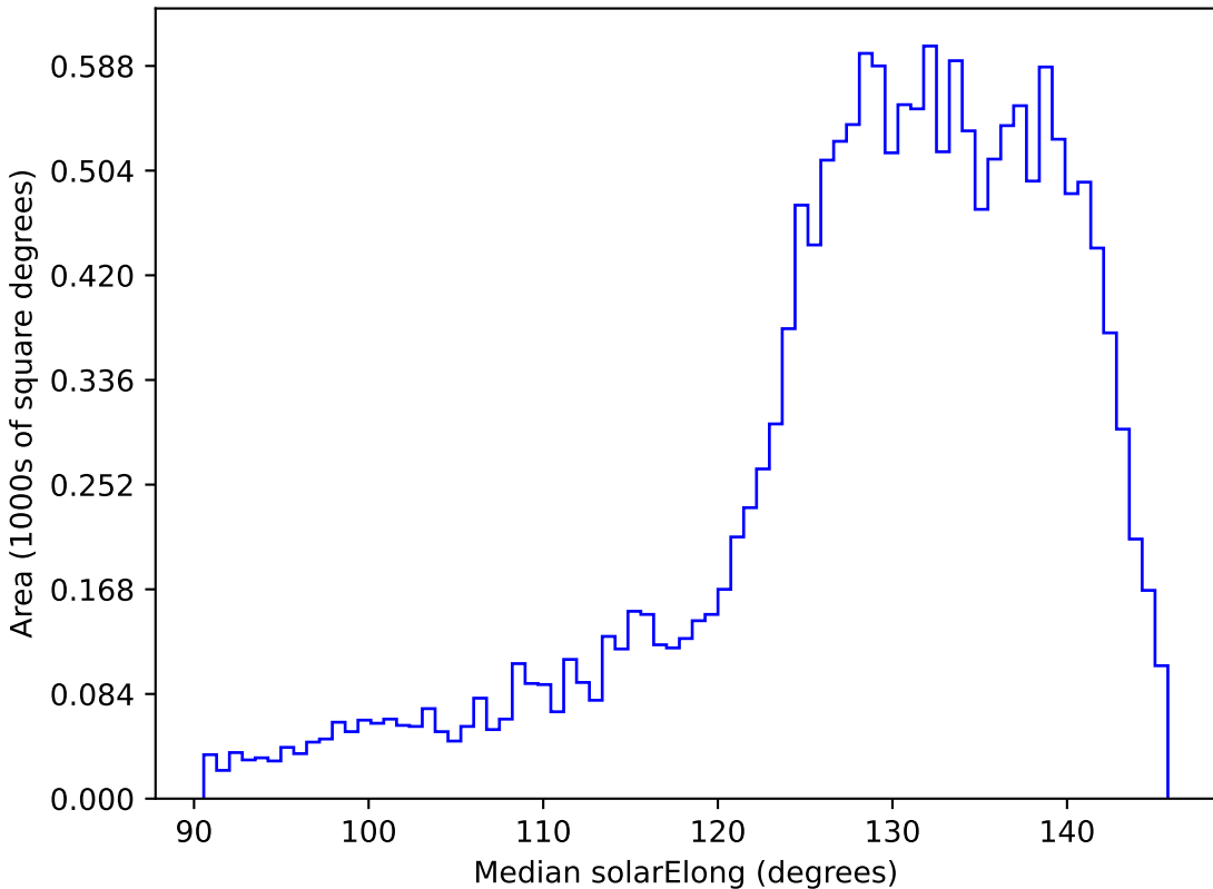
too_ignore_5_4v3.4_10yrs WFD i band: Median solarElong
