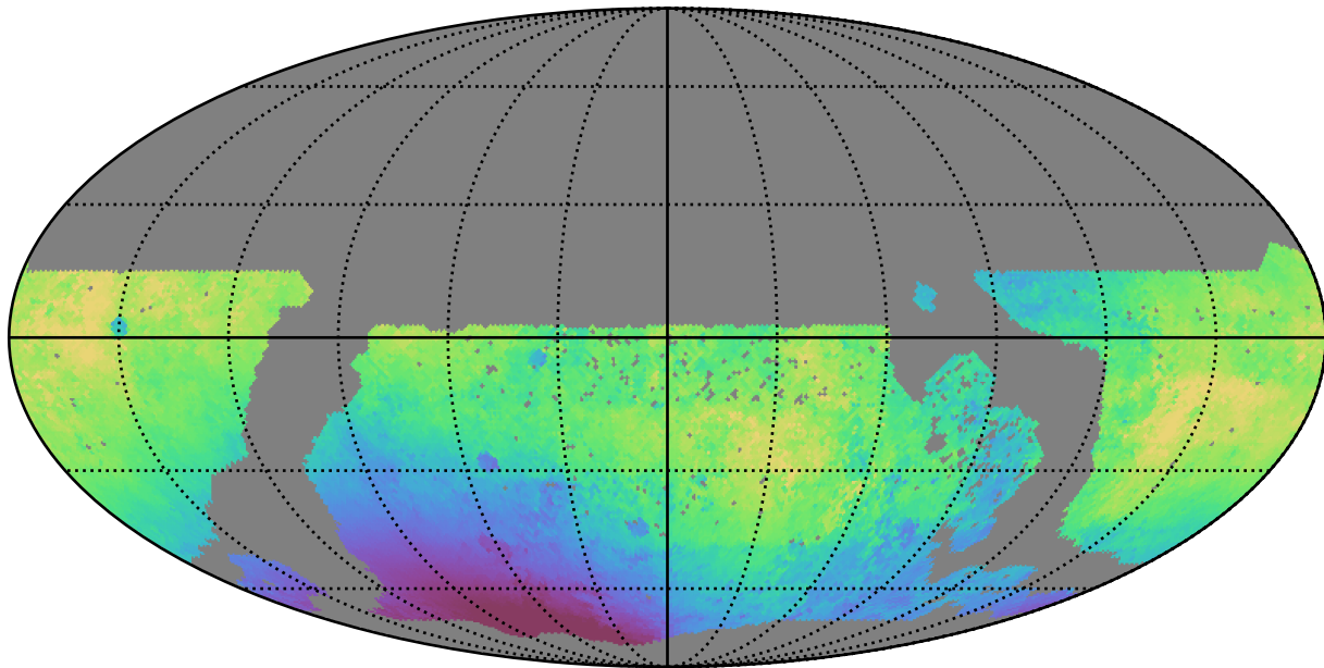
too_ignore_5_4v3.4_10yrs WFD g band: Median solarElong
