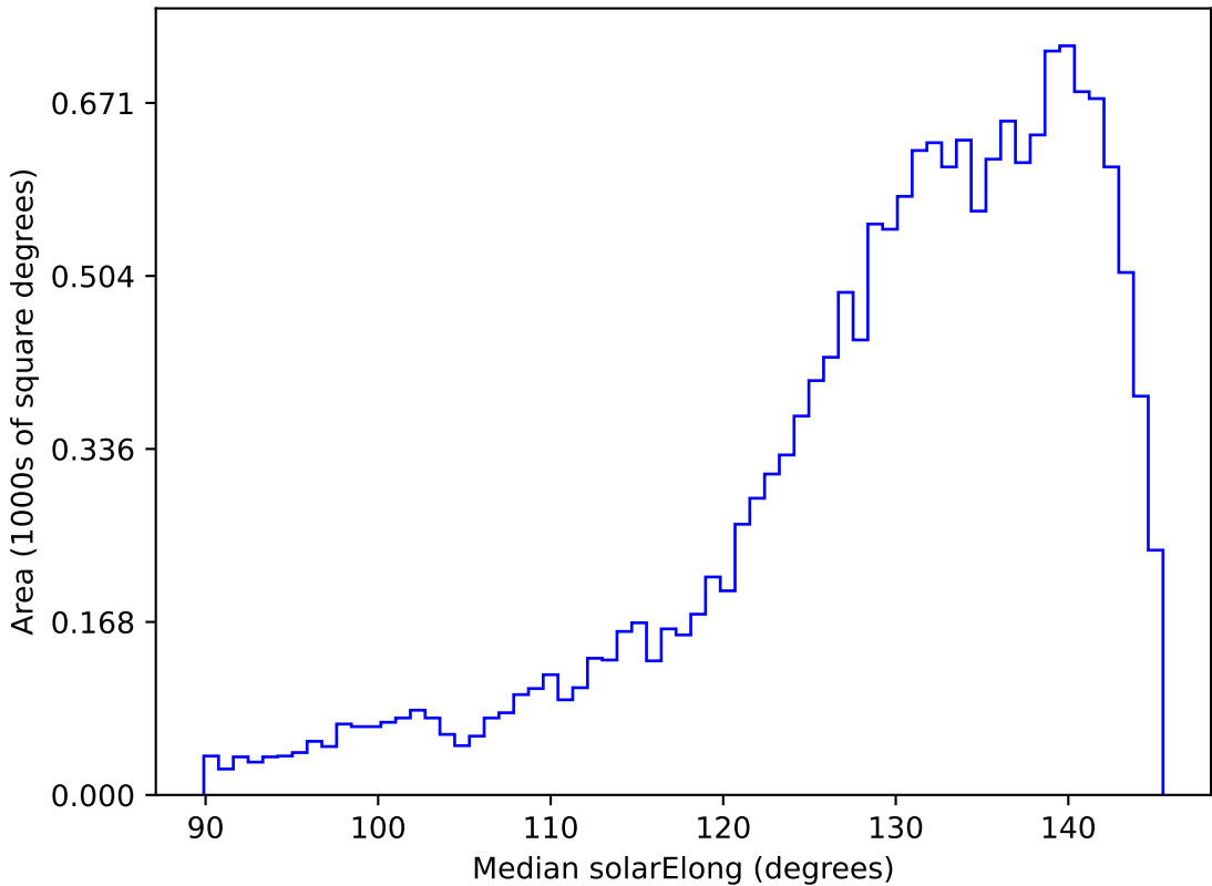
too_ignore_5_4v3.4_10yrs WFD all bands: Median solarElong
