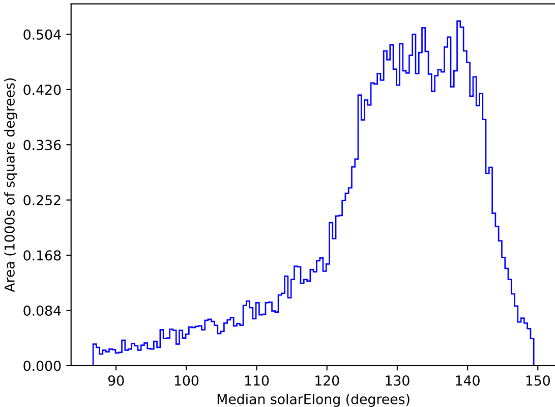
too_ignore_5_4v3.4_10yrs All sky i band: Median solarElong
