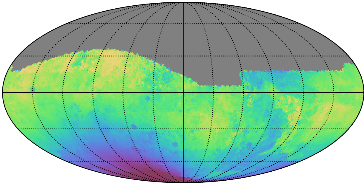
too_ignore_5_4v3.4_10yrs All sky g band: Median solarElong
