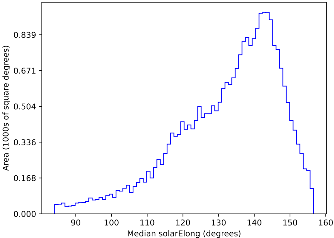
too_ignore_5_4v3.4_10yrs All sky g band: Median solarElong
