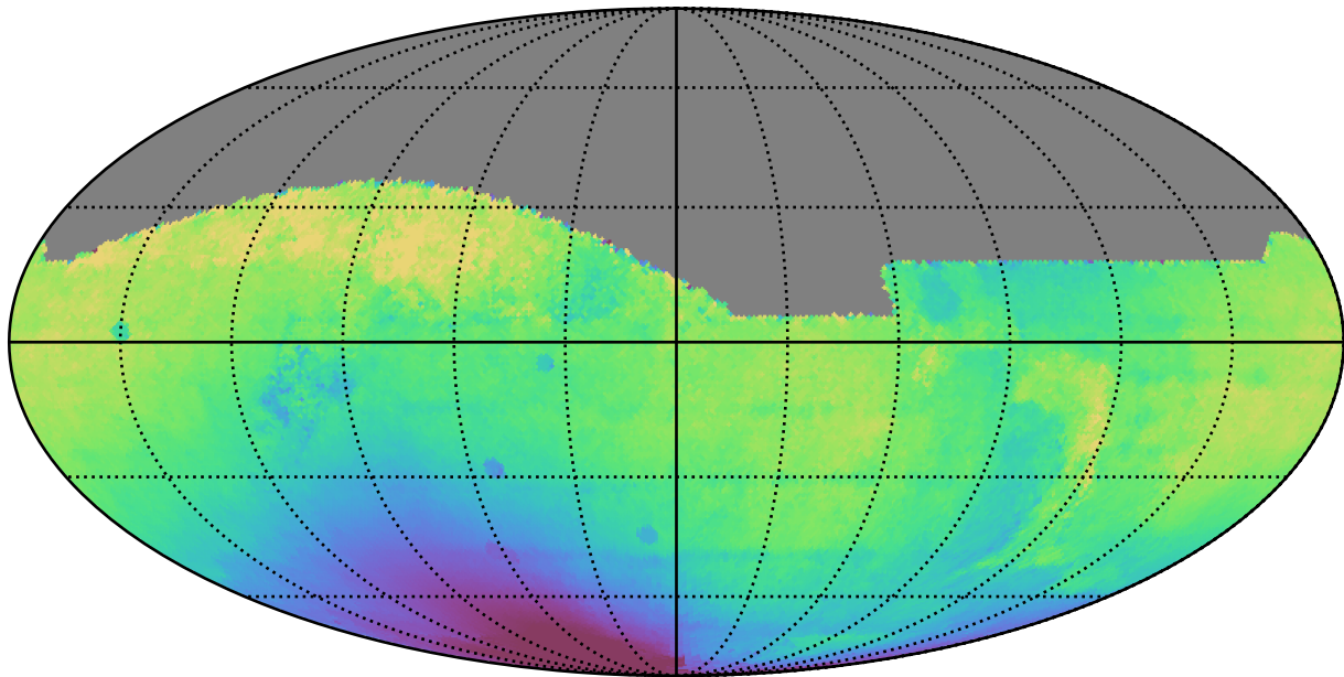
too_ignore_5_4v3.4_10yrs All sky all bands: Median solarElong
