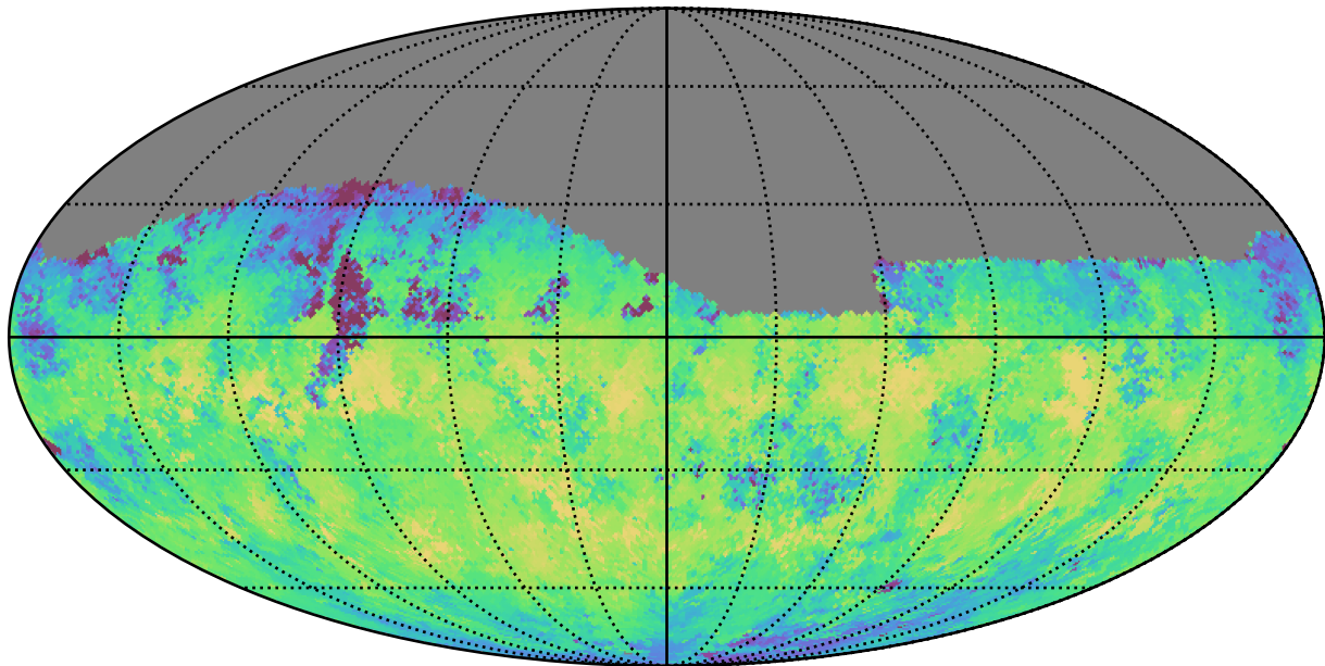
too_ignore_5_4v3.4_10yrs Yr 1 z band: Median skyBrightness
