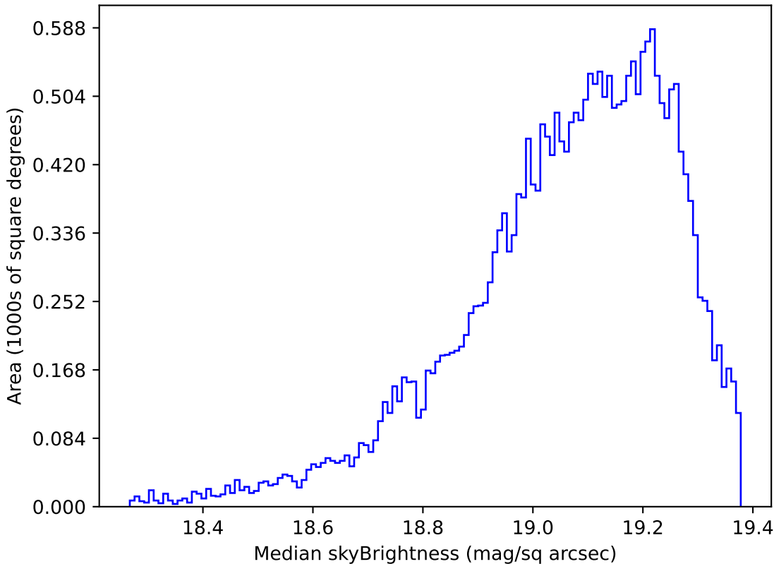
too_ignore_5_4v3.4_10yrs Yr 1 z band: Median skyBrightness
