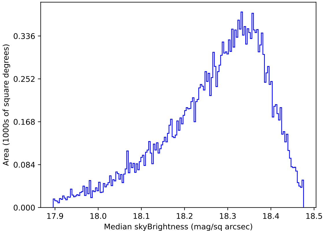
too_ignore_5_4v3.4_10yrs Yr 1 y band: Median skyBrightness
