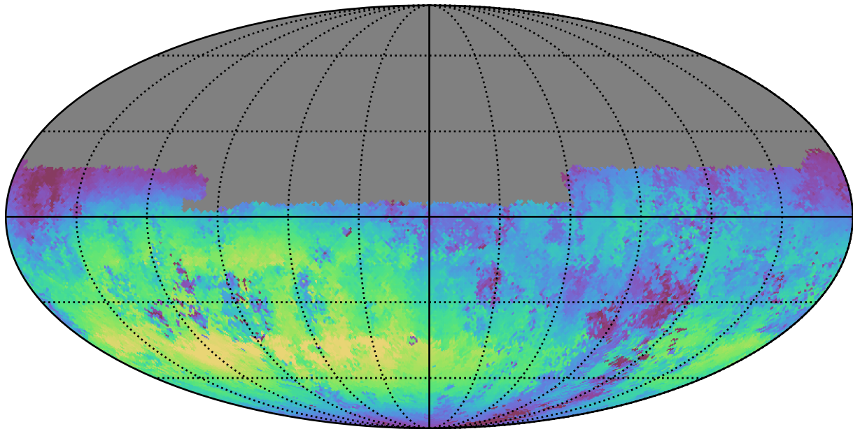
too_ignore_5_4v3.4_10yrs Yr 1 u band: Median skyBrightness
