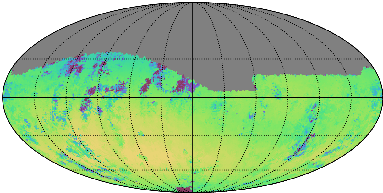
too_ignore_5_4v3.4_10yrs Yr 1 r band: Median skyBrightness
