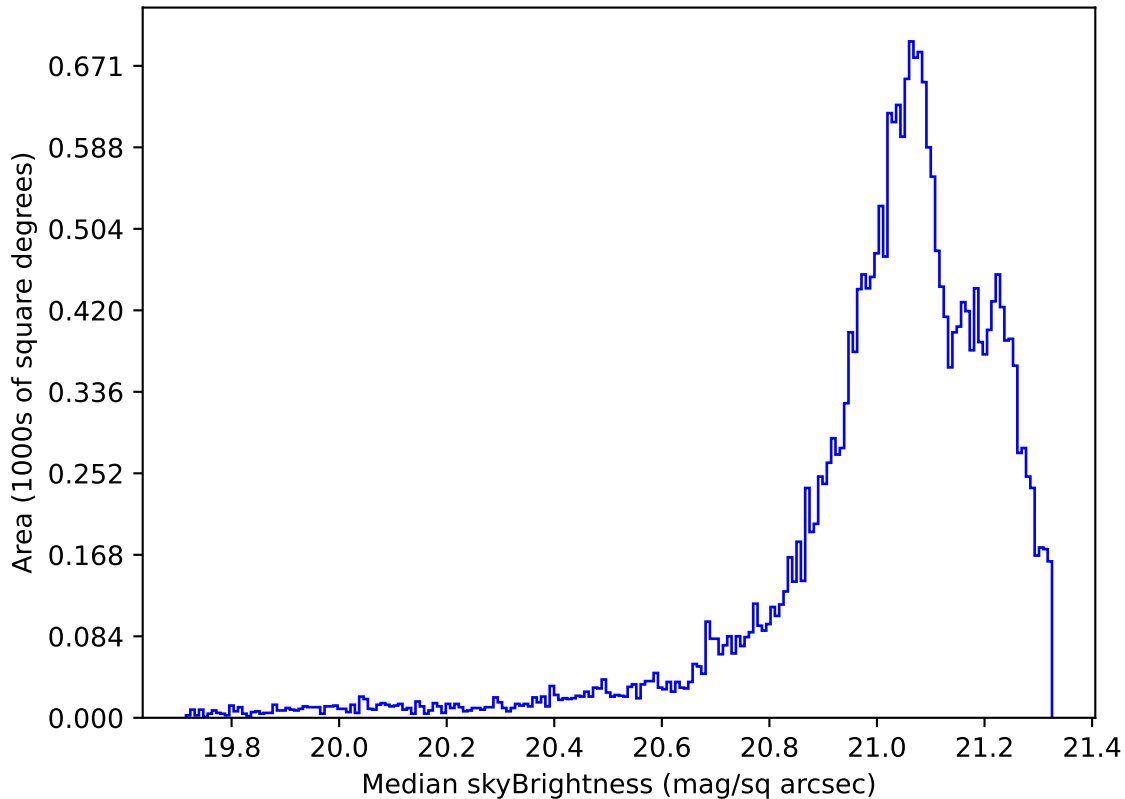
too_ignore_5_4v3.4_10yrs Yr 1 r band: Median skyBrightness
