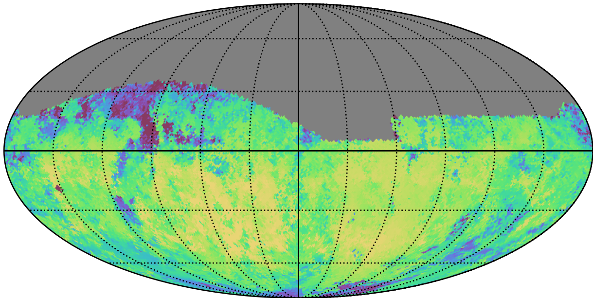
too_ignore_5_4v3.4_10yrs Yr 1 i band: Median skyBrightness
