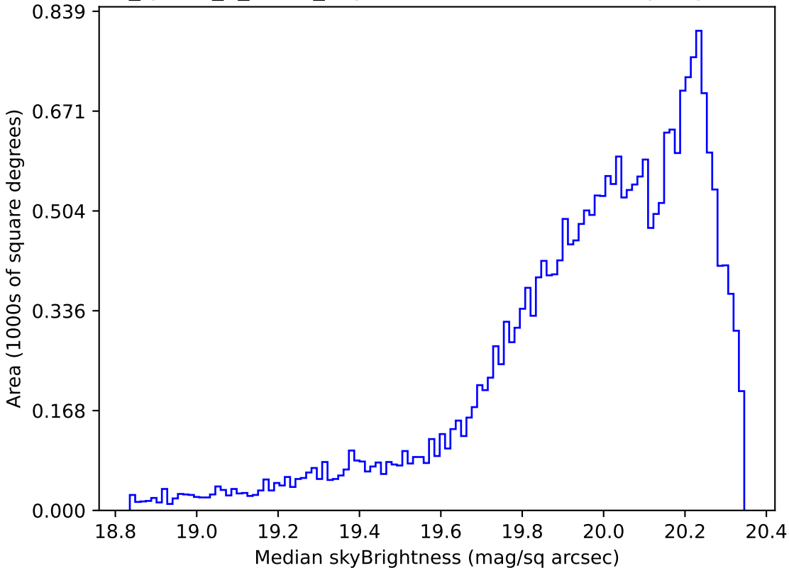
too_ignore_5_4v3.4_10yrs Yr 1 i band: Median skyBrightness
