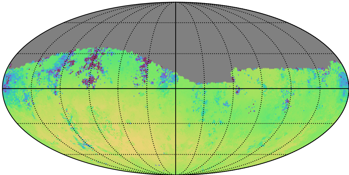
too_ignore_5_4v3.4_10yrs Yr 1 g band: Median skyBrightness
