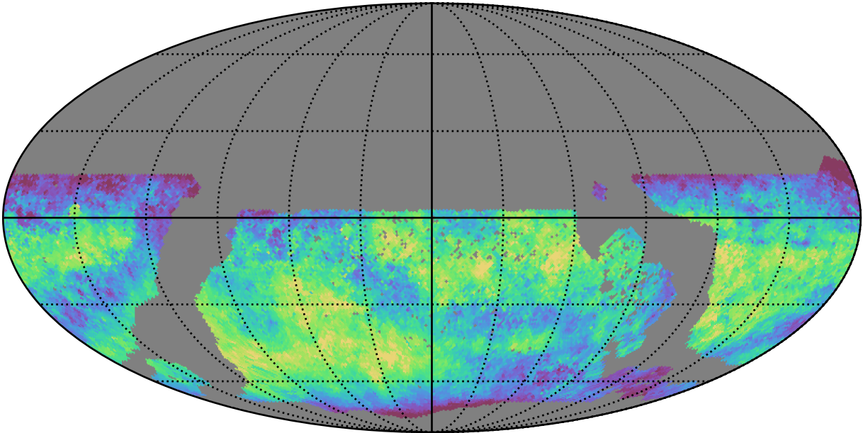
too_ignore_5_4v3.4_10yrs WFD z band: Median skyBrightness
