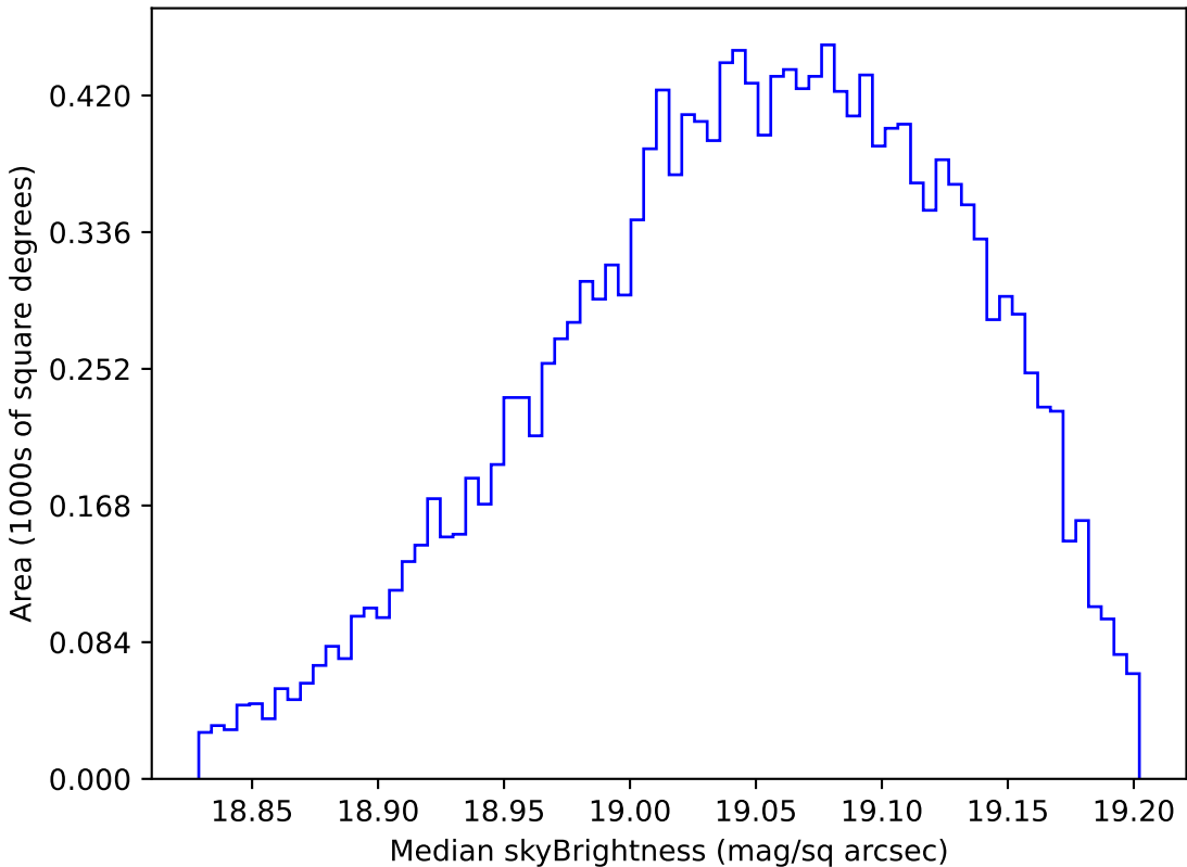
too_ignore_5_4v3.4_10yrs WFD z band: Median skyBrightness
