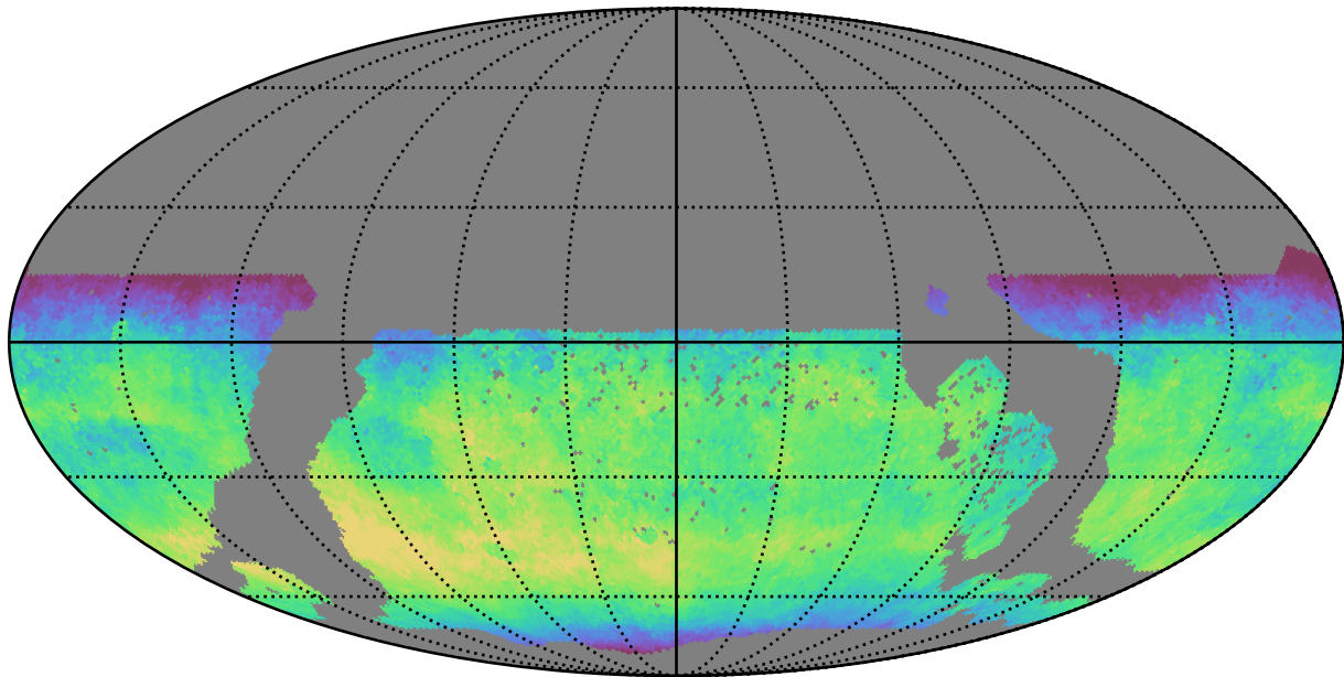
too_ignore_5_4v3.4_10yrs WFD y band: Median skyBrightness
