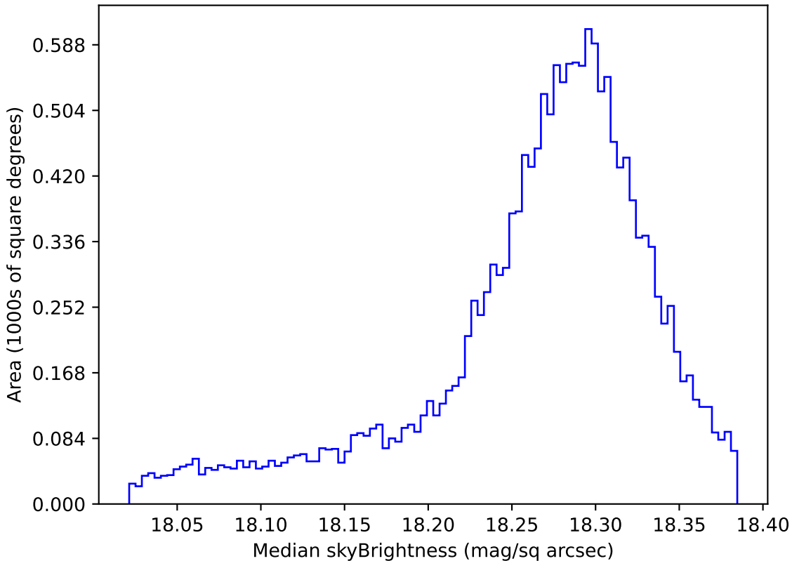
too_ignore_5_4v3.4_10yrs WFD y band: Median skyBrightness
