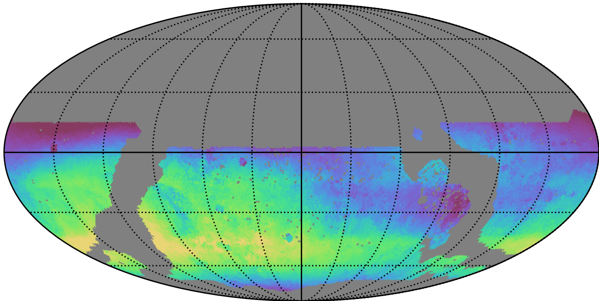
too_ignore_5_4v3.4_10yrs WFD u band: Median skyBrightness
