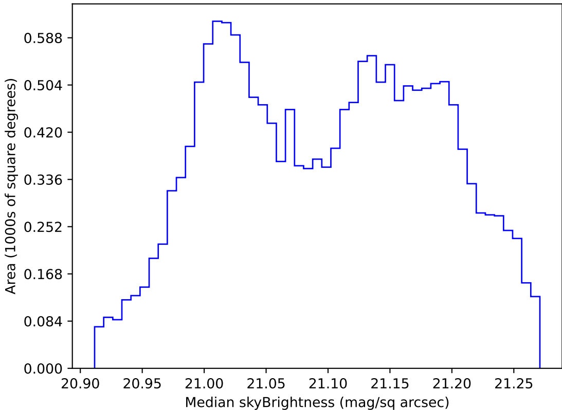
too_ignore_5_4v3.4_10yrs WFD r band: Median skyBrightness
