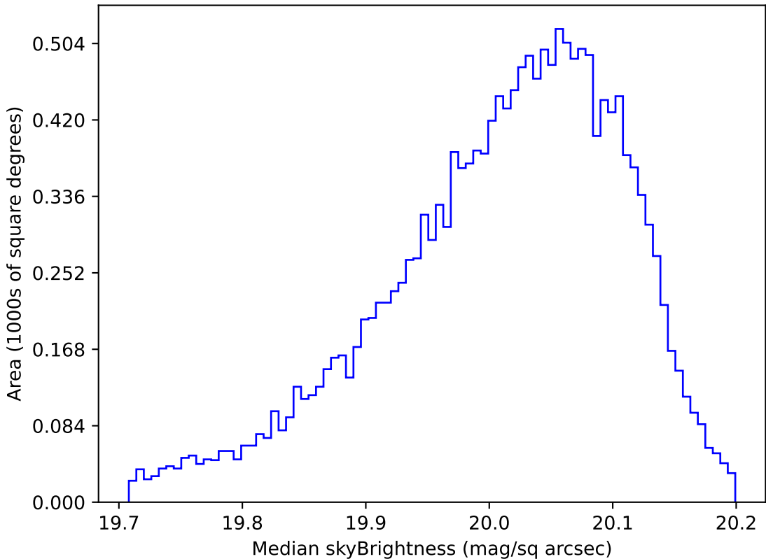
too_ignore_5_4v3.4_10yrs WFD i band: Median skyBrightness
