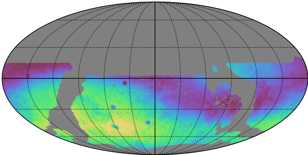
too_ignore_5_4v3.4_10yrs WFD g band: Median skyBrightness
