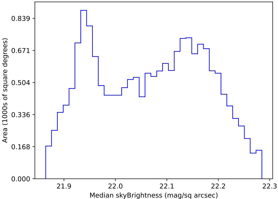
too_ignore_5_4v3.4_10yrs WFD g band: Median skyBrightness
