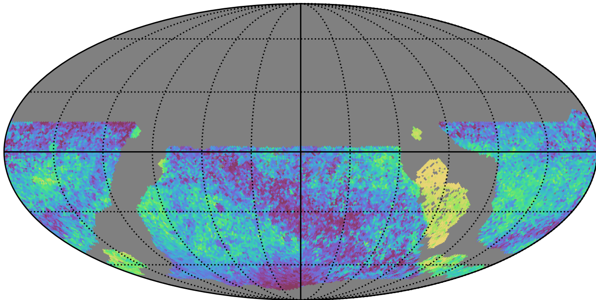
too_ignore_5_4v3.4_10yrs WFD all bands: Median skyBrightness
