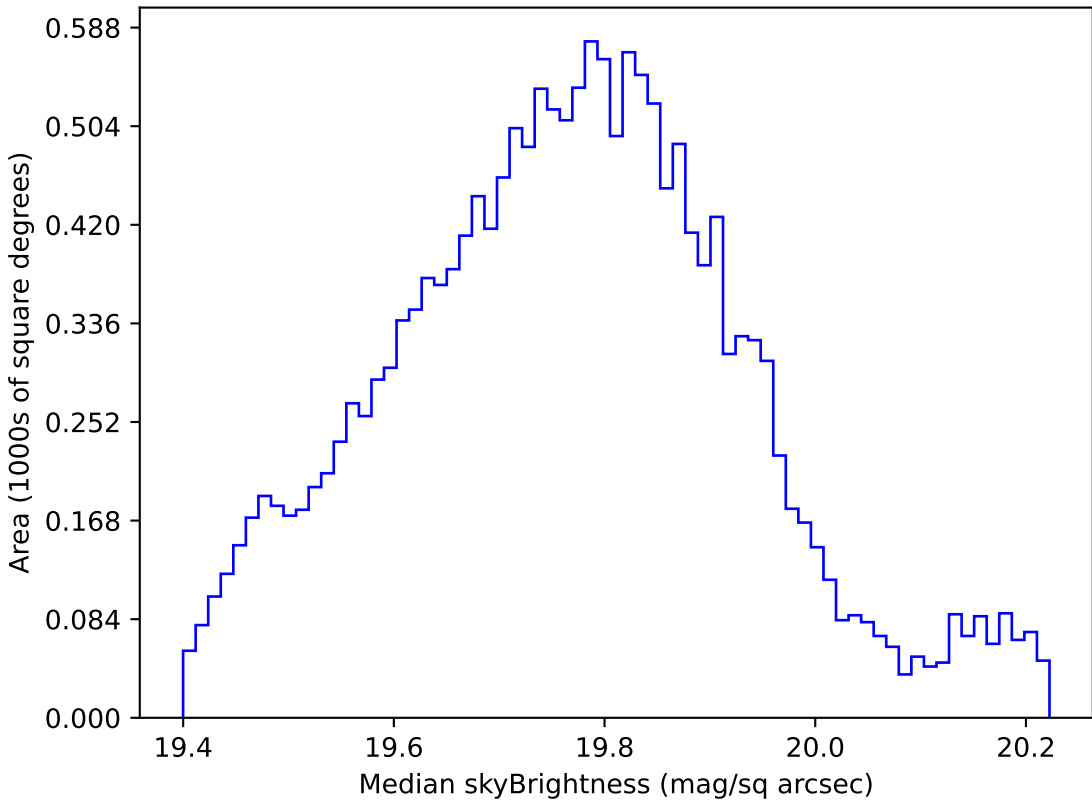
too_ignore_5_4v3.4_10yrs WFD all bands: Median skyBrightness
