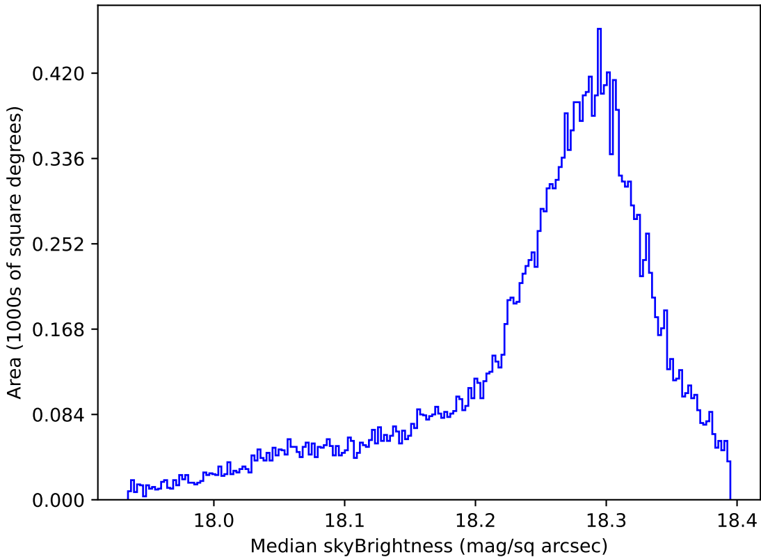
too_ignore_5_4v3.4_10yrs All sky y band: Median skyBrightness
