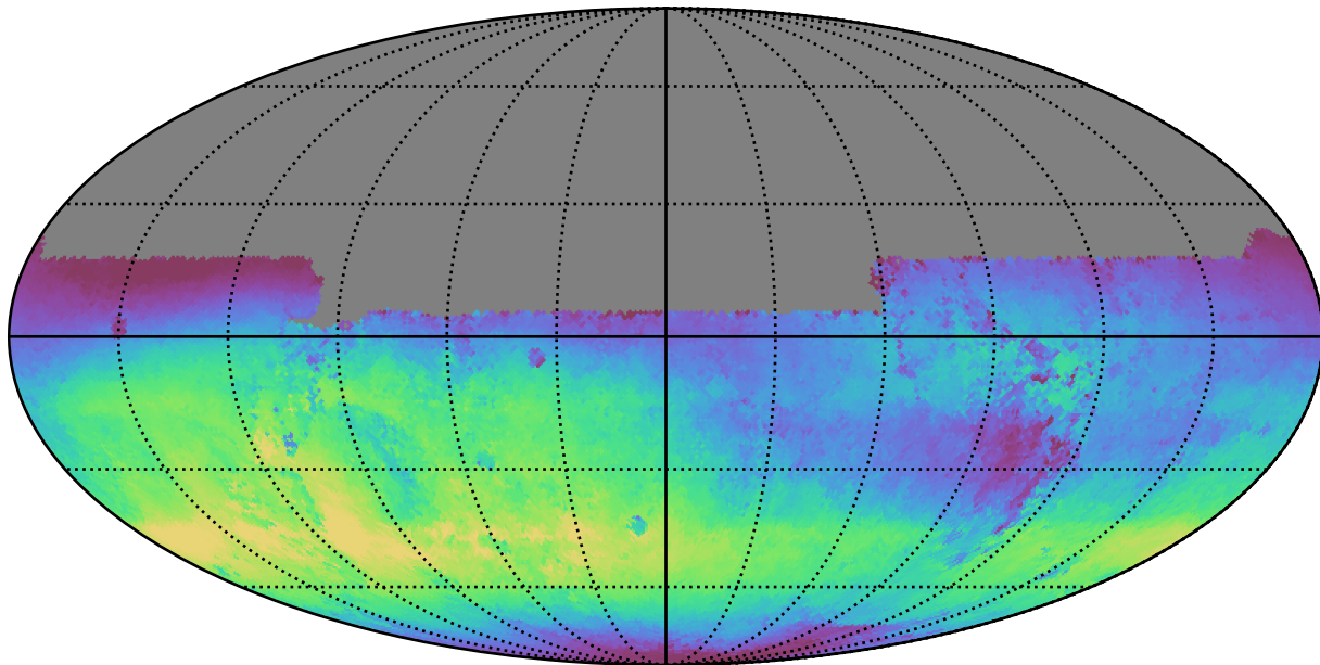
too_ignore_5_4v3.4_10yrs All sky u band: Median skyBrightness
