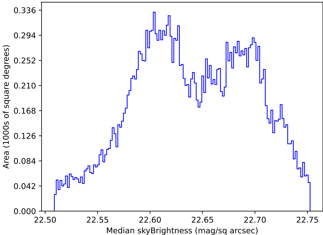
too_ignore_5_4v3.4_10yrs All sky u band: Median skyBrightness
