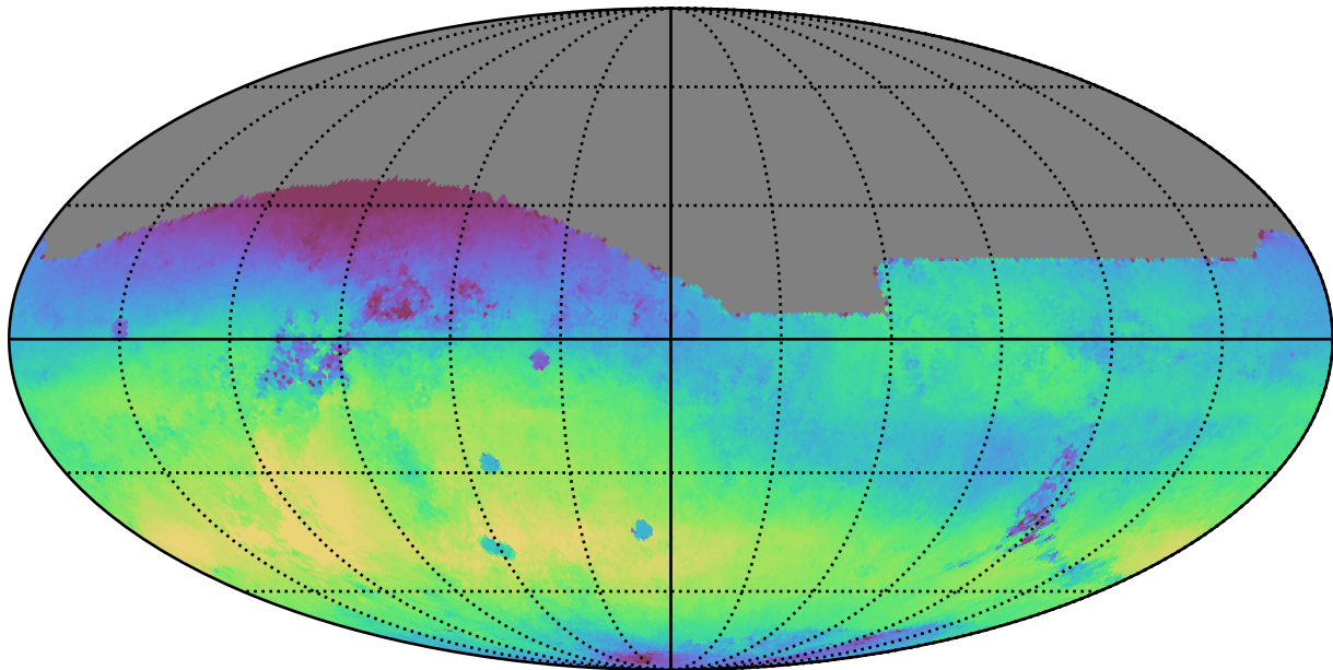
too_ignore_5_4v3.4_10yrs All sky r band: Median skyBrightness
