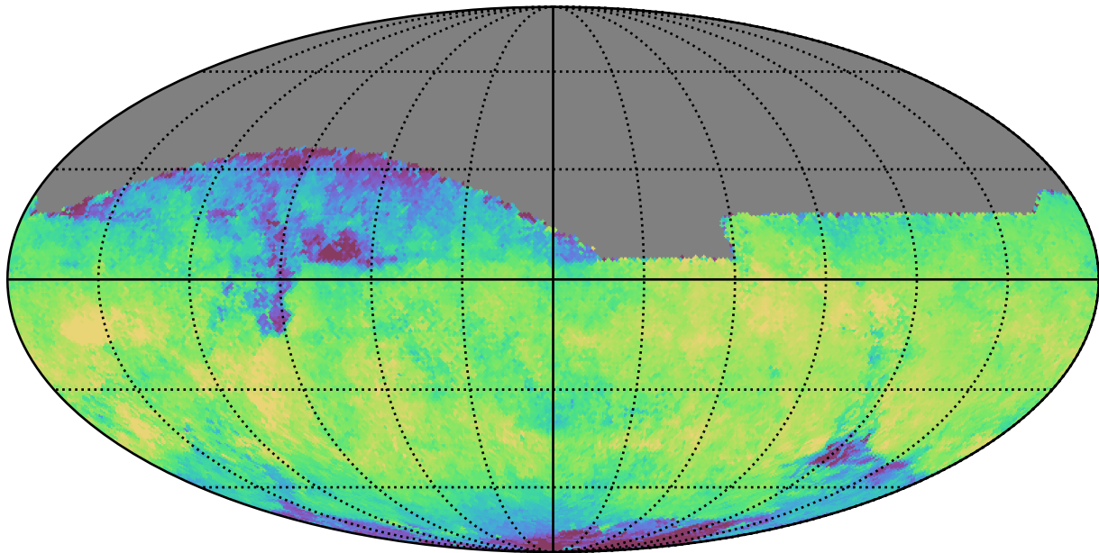
too_ignore_5_4v3.4_10yrs All sky i band: Median skyBrightness
